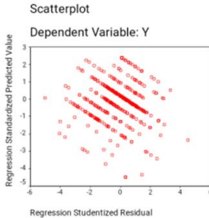
Figure 3. Scatter Plot of Homoscedasticity Testing
